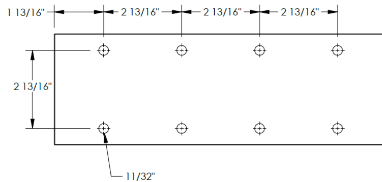
Base (part A) hole location dimensions
